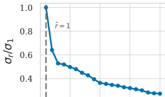
System Prompt
