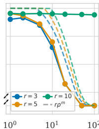
(b) Varying rank r n=100, \rho \approx 0.7
