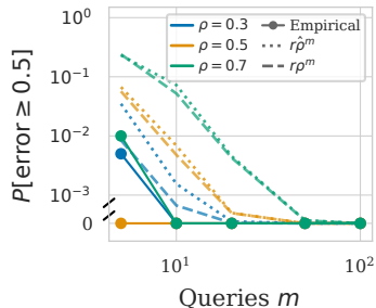
(g) Predicted vs empirical r=1, n=100
