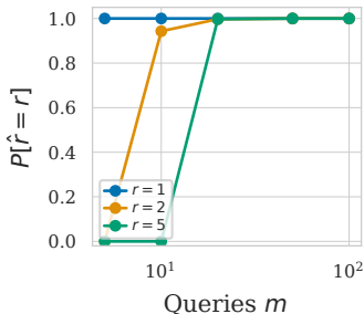
(e) Estimating rank \rho=0.7, n=100
