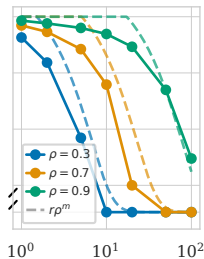
(f) Estimating \rho r=1, n=100
