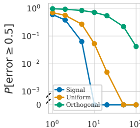
(e) Estimating rank \rho=0.7, n=100
