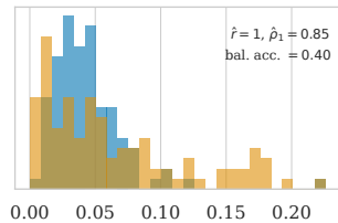
System Prompt
