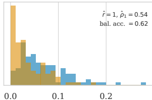
bge-large-en-v1.5
