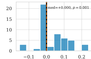
System Prompt
