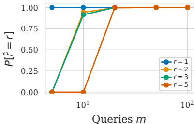
(e) Estimating rank \rho=0.7, n=100
