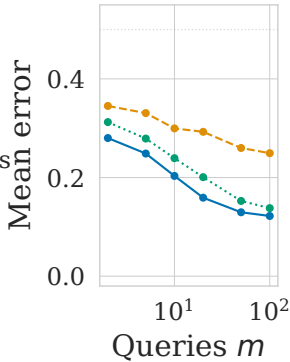
(b) Error vs m ( n=50 )
