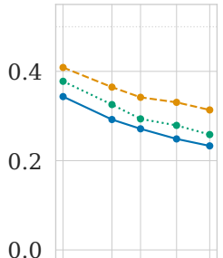
(c) Error vs n ( m=5 )
