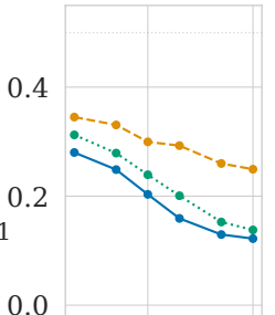
(b) Error vs m ( n=50 )
