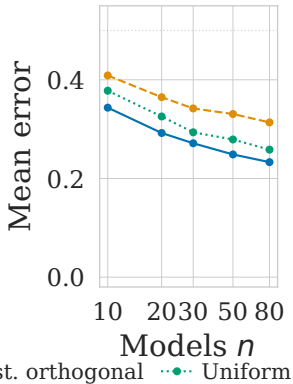
(c) Error vs n ( m=5 )
