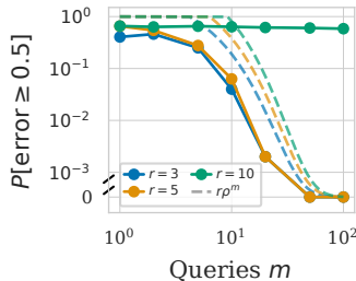
(e) Estimating rank \rho=0.7, n=100
