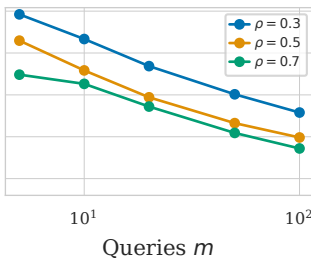
(f) Estimating \rho r=1, n=100
