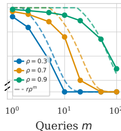
(f) Estimating \rho r=1, n=100
