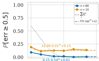
\mathbb{P}[\text{err} \geq 0.5] vs m
