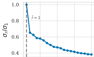
Singular values of \tilde{E}
