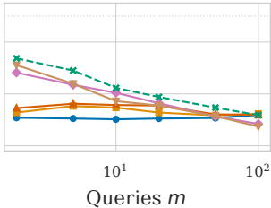
System Prompt
