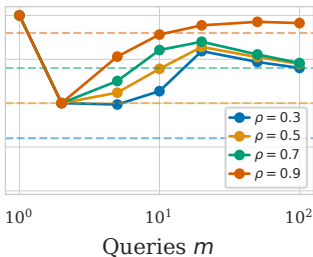
(f) \hat{\rho} recovery r=5, n=100
