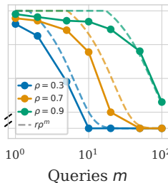
(f) \hat{\rho} recovery r=5, n=100
