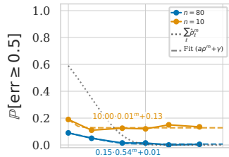
P[\text{err} \geq 0.5] vs m
