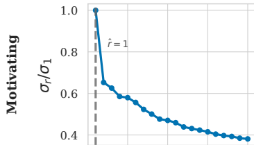
Singular values of \tilde{E}
