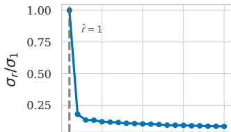
Singular values of E
