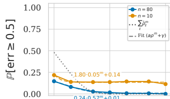
P[\text{err} \geq 0.5] vs m
