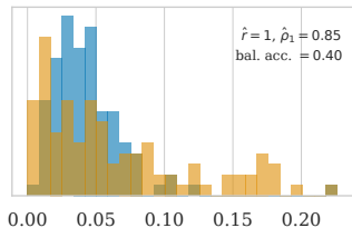
System Prompt
