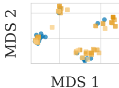
Orthogonal queries, m=5
