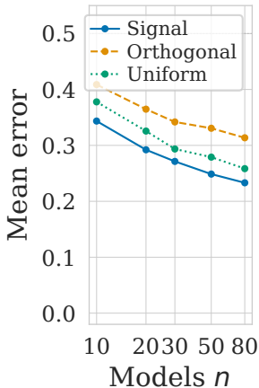
(c) Error vs n ( m=5 )
