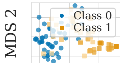
(a) Signal queries, m=5
