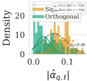
GMM on |\hat{\alpha}_{q,\ell}| Estimated & Fitted Errors
