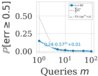
GMM on |\hat{\alpha}_{q,\ell}| Estimated & Fitted Errors
