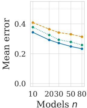
(c) Error vs n ( m=5 )
