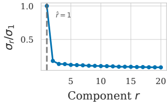
Singular values of E
