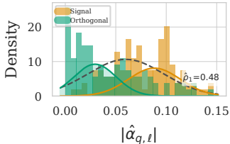
GMM on |\hat{\alpha}_{q,\ell}|
