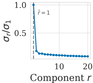
Singular values of E
