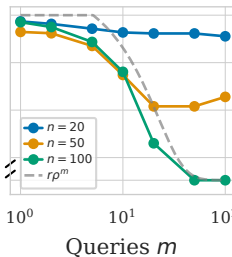
(f) \hat{\rho} estimation error r=5, n=100
