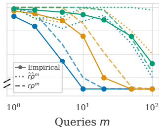
(g) Predicted vs empirical r=5, n=100
