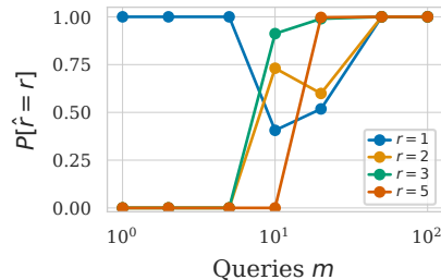
(e) Rank recovery \rho=0.7, n=100
