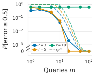
(e) Rank recovery \rho=0.7, n=100
