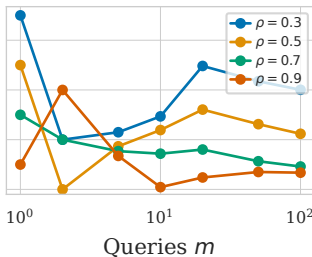
(f) \hat{\rho} estimation error r=5, n=100
