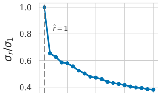
Singular values of E
