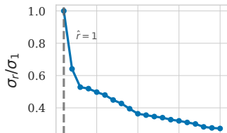
System Prompt
