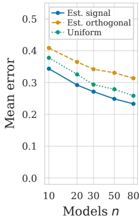
(c) Error vs n ( m=5 )
