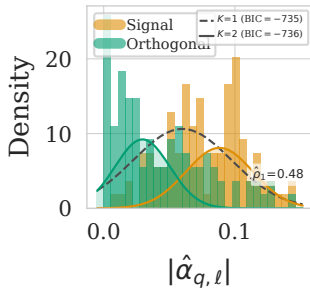
GMM on |\hat{\alpha}_{q,\ell}|
