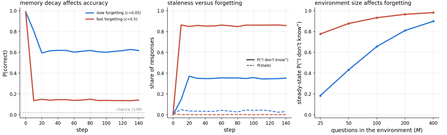
Figure 1: Epistemic collapse. Warm-started systems on the measured-gate proxy of Sec. 2 (real gpt-4o-mini version forthcoming): every agent is seeded at t = 0 with the current truth of all M = 50 questions; two populations differ only in memory decay (20 seeds each; 20-question probe panel). Left: accuracy collapses from a perfect start to a decay-determined plateau; dotted line = chance ( 1/M ). Center: the failure mass split into its two forms — abstention (solid) vs. stale answers (dashed); forgetting dominates, and staleness is carried by the fastest questions. Right: steady-state abstention grows with the number of questions the environment holds ( M , cold-start toy runs): breadth crowds memory, silencing the population regardless of decay.
