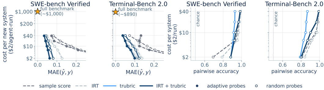
Figure 5: Evaluation cost per target system (at a nominal $2 per execution) to reach a given MAE (left two panels) and a given pairwise ranking accuracy on system pairs separated by at least 0.05 (right two panels). The star marks full-benchmark evaluation: exact scores at full cost.
