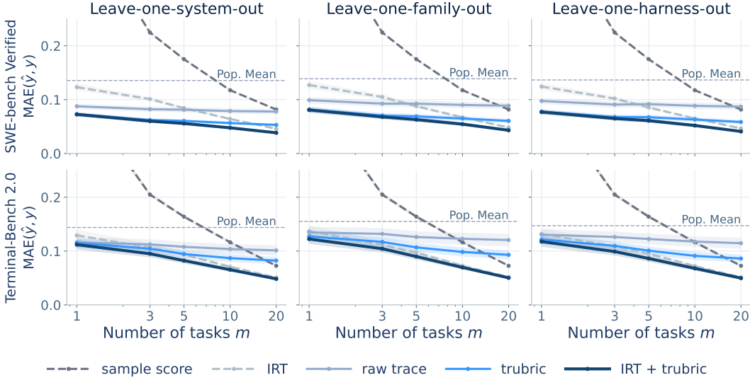
Figure 3: MAE of benchmark-score estimators as a function of the task budget m (random task selection, B = 50 shared draws, \pm 1 SEM bands) on SWE-bench Verified (top) and Terminal-Bench 2.0 (bottom) under three reference-exclusion protocols of increasing conservatism.
