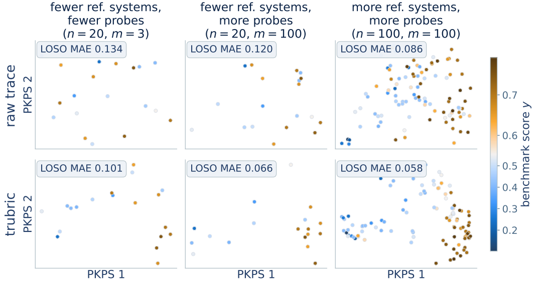
Figure 2: Two-dimensional PKPS representations of 107 SWE-bench Verified systems, colored by benchmark score (gold high, blue low), for raw-trace embeddings (top) and TRUBRIC embeddings (bottom) as the number of reference systems n and tasks m grows. Panels within a row are Procrustes-aligned; badges report leave-one-system-out MAE of a k NN predictor in each panel.
