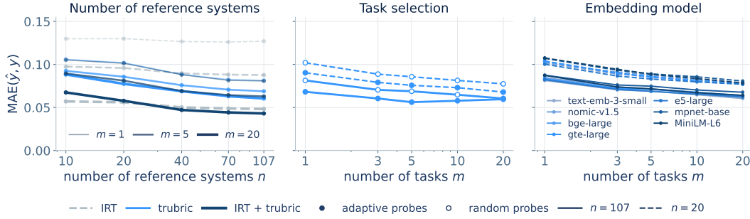
Figure 4: Ablations under leave-one-family-out evaluation on SWE-bench Verified. (a) Effect of the number of reference systems n for m \in \{1, 5, 20\} tasks (line weight). (b) Random (open) vs. adaptive (filled) task selection for TRUBRIC geometry with n = 107 (solid) and n = 20 (dashed) reference systems. (c) Effect of the text encoder on TRUBRIC geometry.
