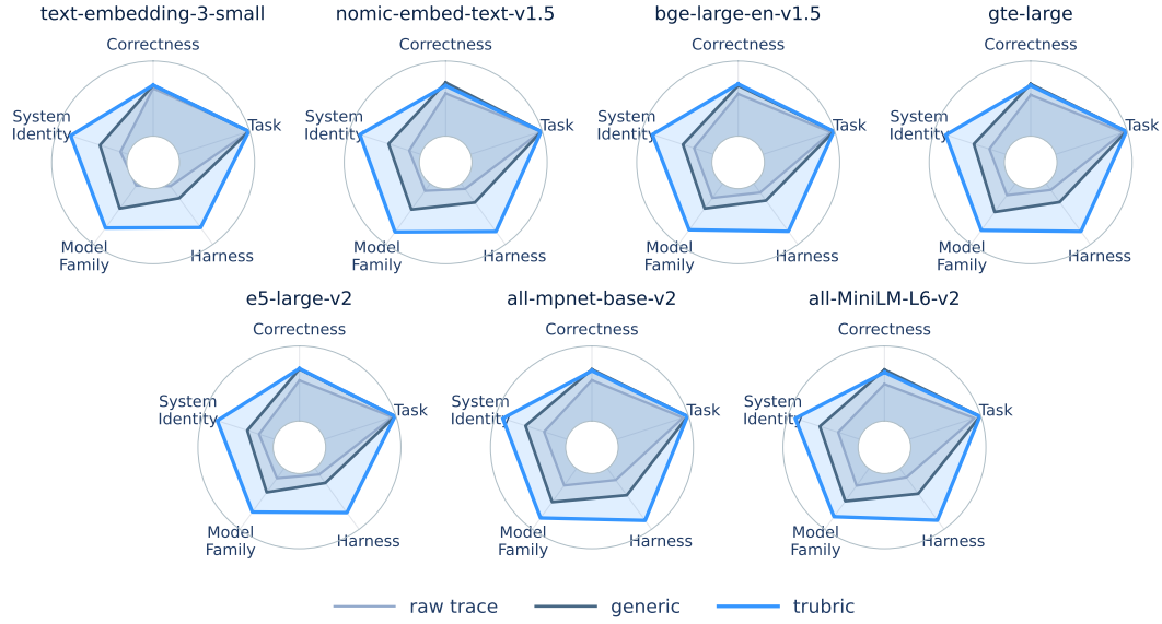
Figure 1: Held-out balanced accuracy of linear probes for five trace attributes, chance-normalized so that chance sits at the center and better-for-evaluation is outside: content attributes (Correctness, Task) plot recoverability and system-metadata attributes (Harness, Model Family, System Identity) plot its complement. One panel per text encoder; raw traces vs. generic-rubric vs. TRUBRIC summaries.
