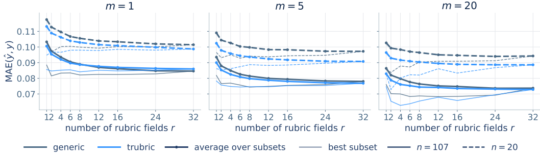
Figure 6: Effect of rubric size r on MAE for generic and task-specific (TRUBRIC) rubrics, averaged over up to 200 random size- r subsets of a 32-field bank (thick: mean \pm 1 SEM; thin: best subset per size), for m \in \{1, 5, 20\} tasks and reference libraries of n = 107 (solid) and n = 20 (dashed) systems.
