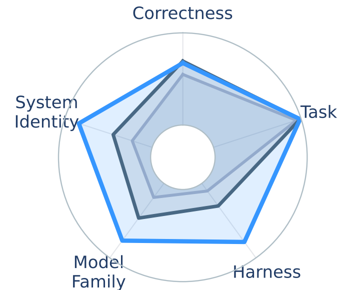
all-MiniLM-L6-v2
