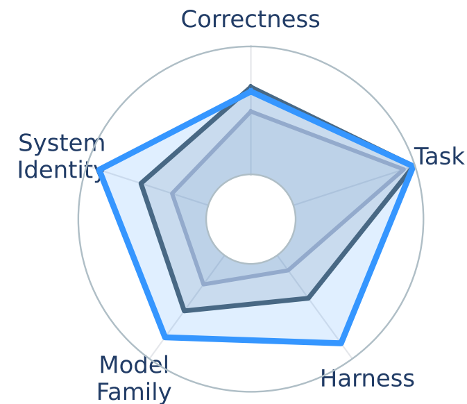
all-MiniLM-L6-v2
