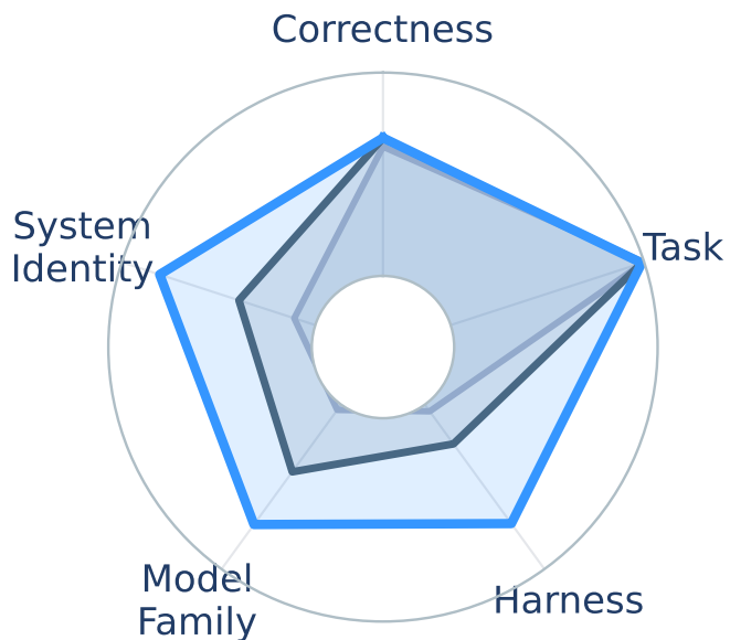
e5-large-v2
