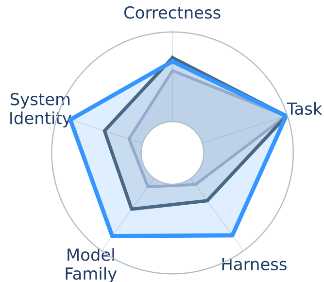
e5-large-v2
