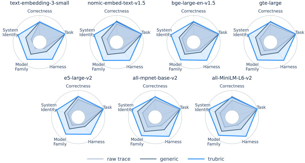
Figure 1: Comparisons of the properties of three different methods for embedding executed task traces across seven different off-the-shelf text encoders: embedding the raw trace, embedding a structured summary based on a generic rubric, and embedding a structured summary based on a task-specific rubric. As measured by the balanced accuracy of held-out linear probes, described in Section 3, the embedding of the task-specific summary is better at removing undesirable signal while preserving relevant signal across all seven encoders.
