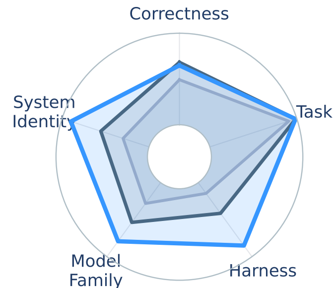
all-MiniLM-L6-v2
