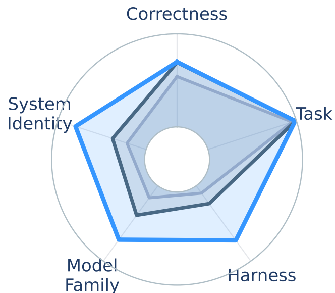
e5-large-v2
