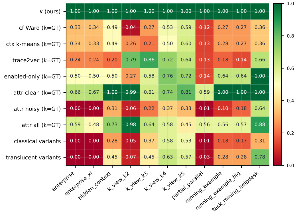
(b) recovery ARI, k = \text{GT} (cf. Fig. 2)
