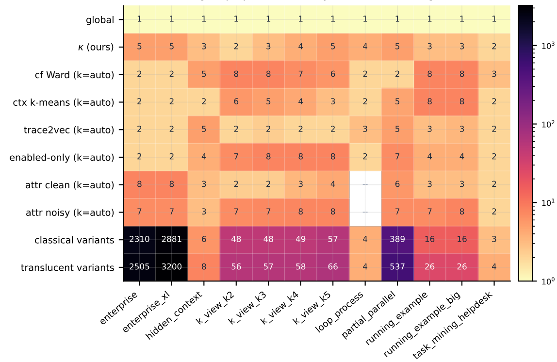
(a) groups produced, k by silhouette (cf. Fig. 1)
