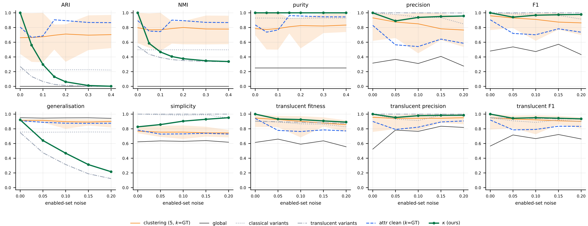
ServiceDesk case study: every approach vs. enabled-set noise
