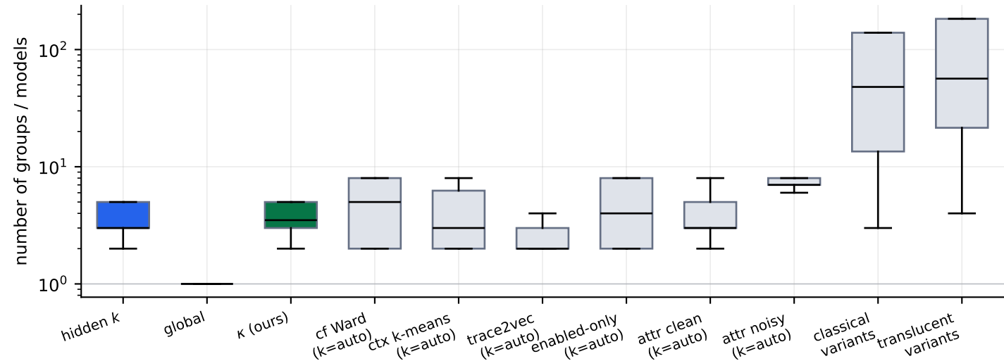
Separation: groups produced per method (log scale; clustering with k by silhouette)
