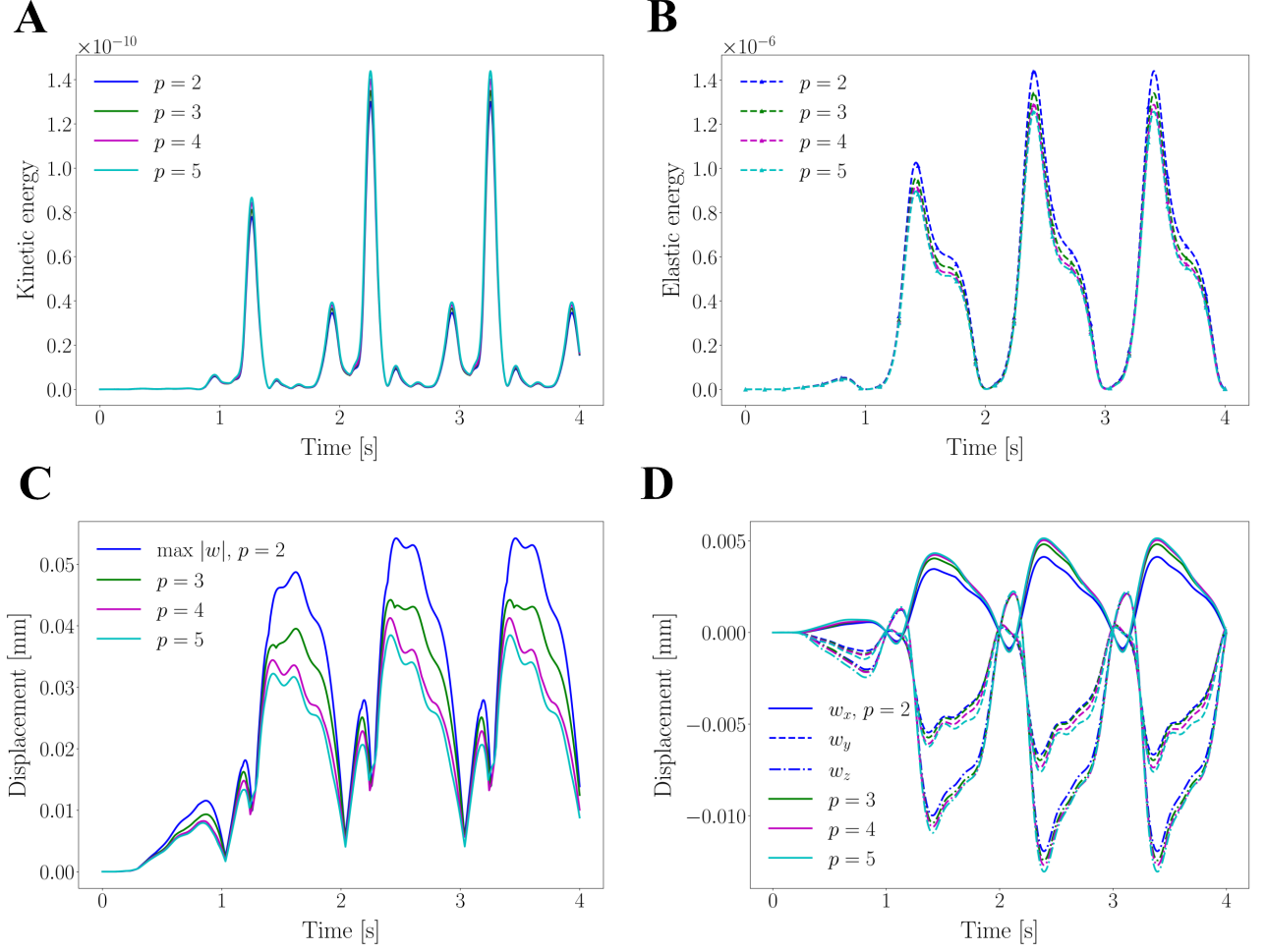
Figure 11: Refinement study when refining element degree ( p ) for the tissue deformation model on the standard mesh (mesh 1).
