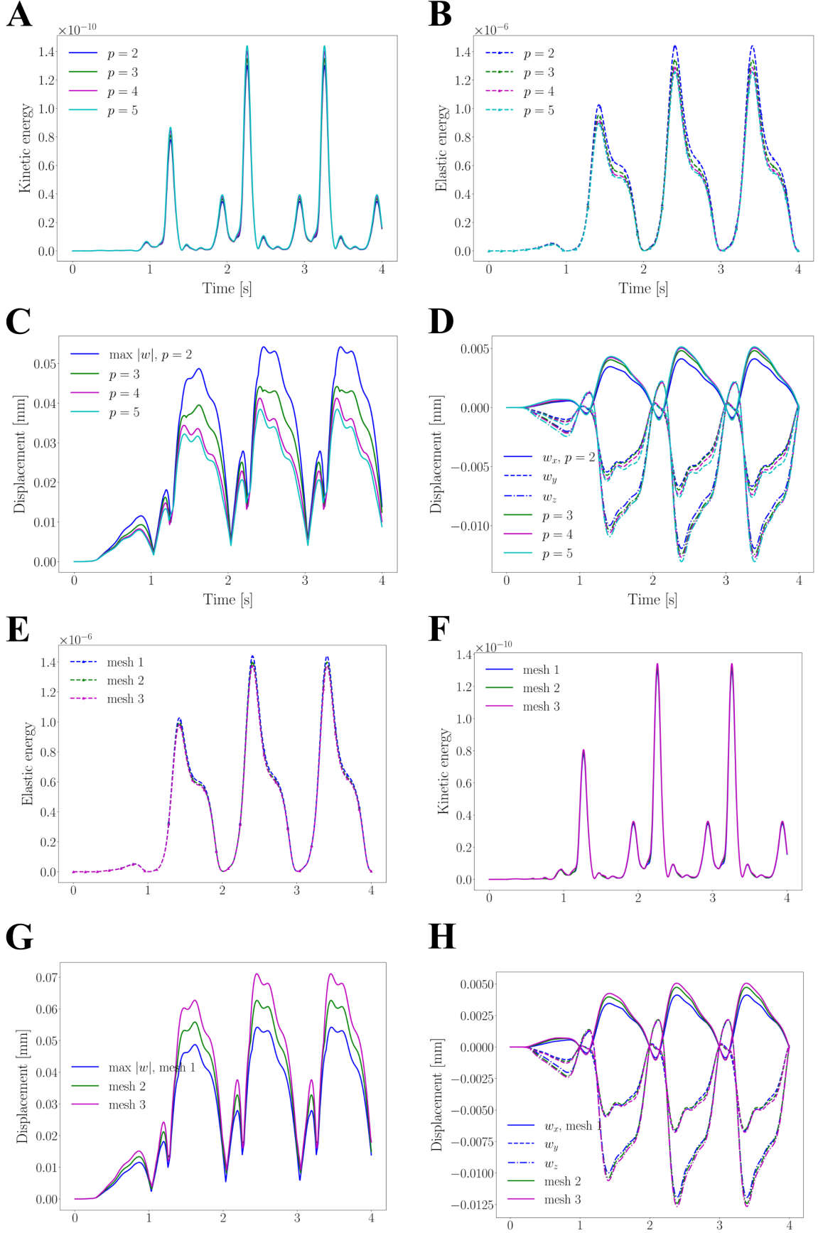
Figure 11: Convergence under A–D. Refinement study when refining element degree ( p ) refinement for the linear elastodynamics-tissue deformation model on the standard mesh (mesh 1). E–H. Refinement study when refining the mesh for the tissue deformation model using quadratic polynomial basis functions ( p=2 ). The standard mesh is mesh 1.
