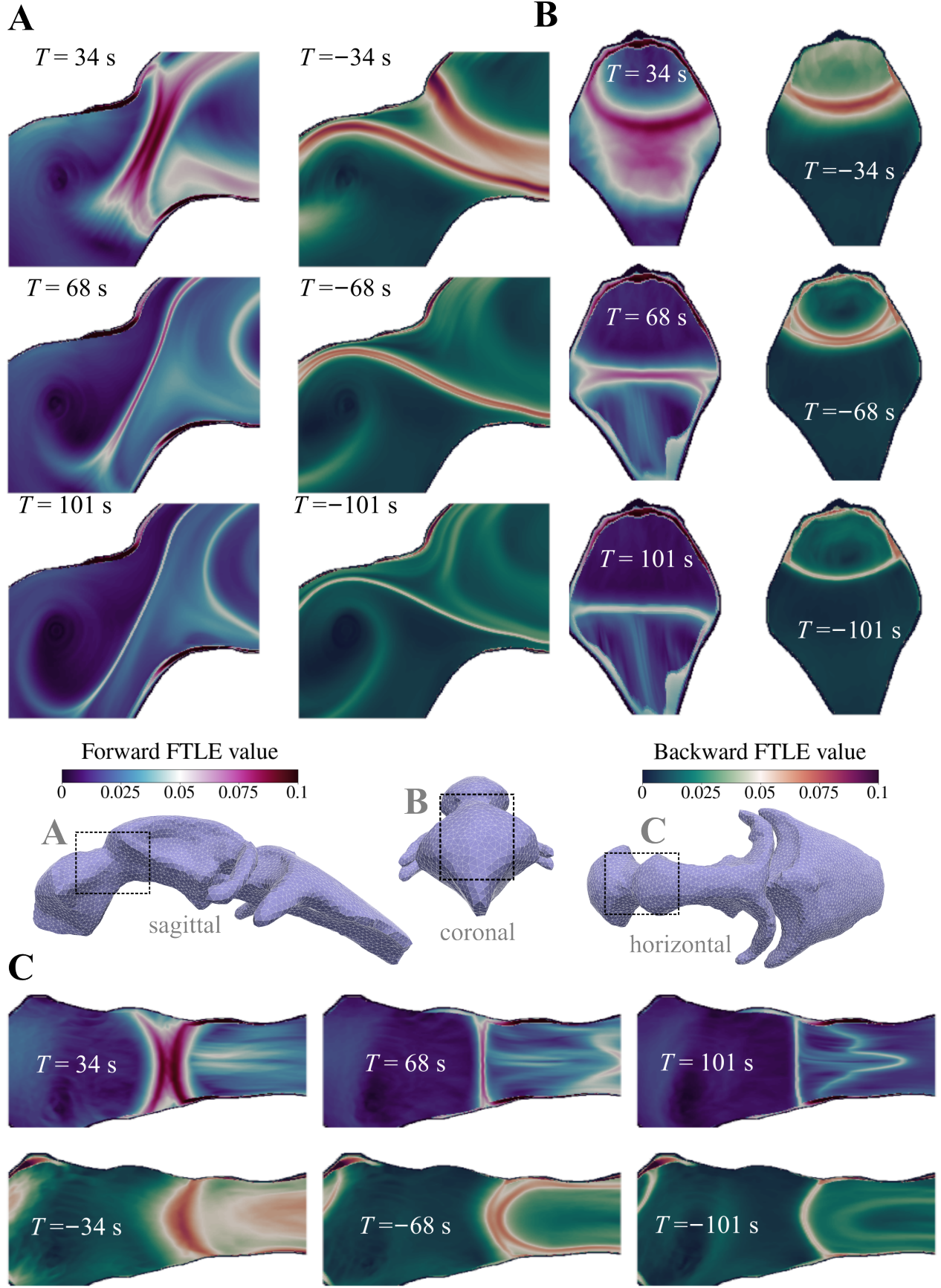
Figure 10: FTLE fields for integration times T = \pm\{34, 68, 101\} s in embryonic zebrafish brain ventricles. The FTLE fields were computed in a box-3D box-formed section of the interventricular duct connecting the anterior and middle ventricles. We present 2D slices extracted from the 3D FTLE field computations: Sagittal ( A ), coronal ( B ) and horizontal slices ( C ) in the center of the 3D box used for computation are displayed. Common legends for all forward-in-time and all backward-in-time fields.
