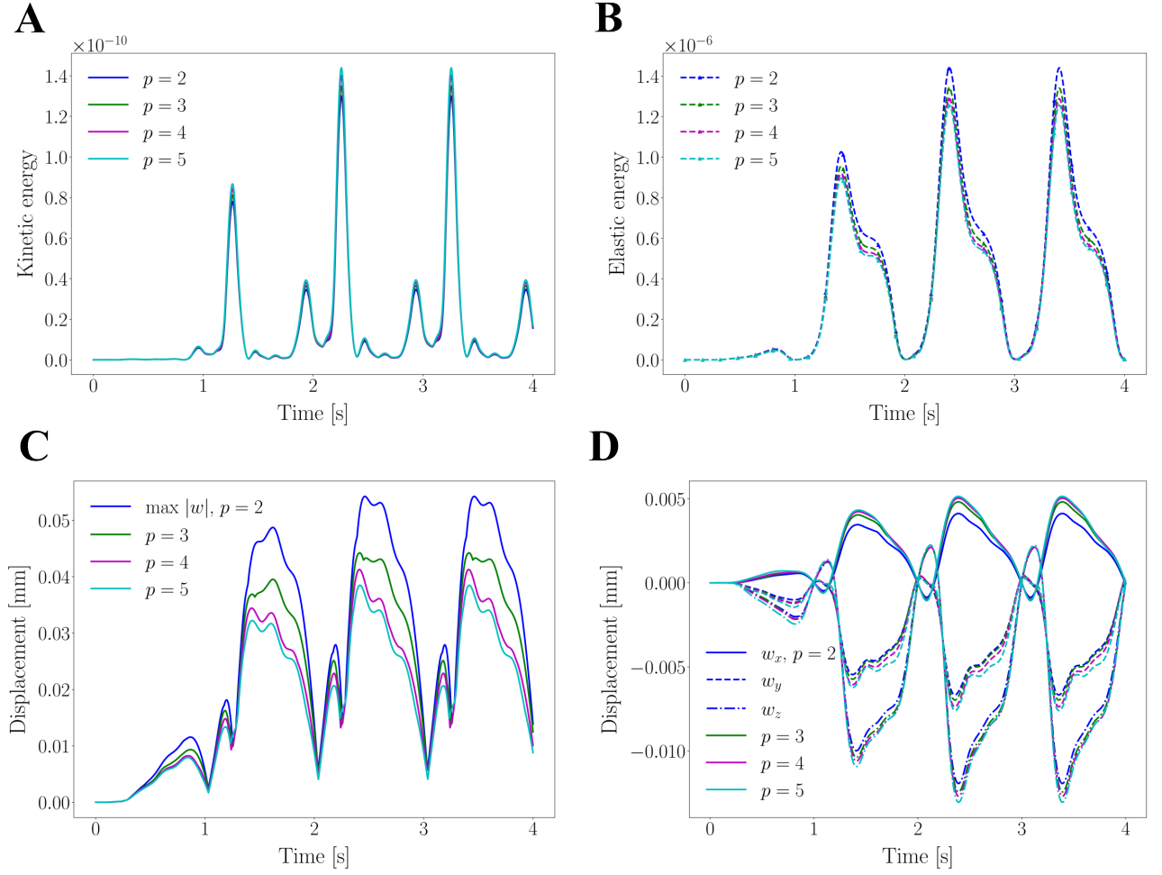
Figure 11: Convergence under Refinement study when refining element degree ( p ) refinement for the linear elastodynamics tissue deformation model on the standard mesh (mesh 1).
