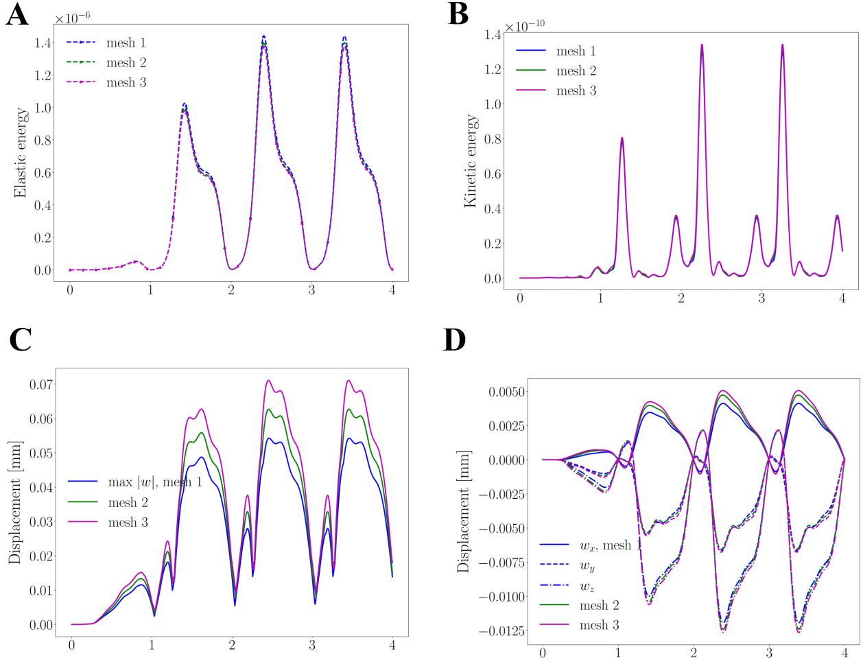
Figure 12: Convergence under Refinement study when refining the mesh refinement for the linear elastodynamics tissue deformation model using quadratic polynomial basis functions ( p = 2 ). The standard mesh is mesh 1.
