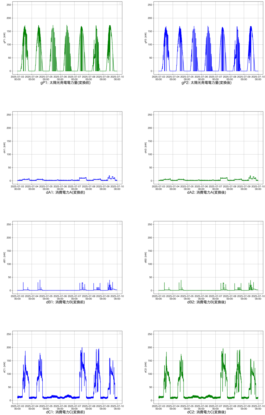
Figure 5.2: Optimization Results (Linear Programming Model) – Page 1
