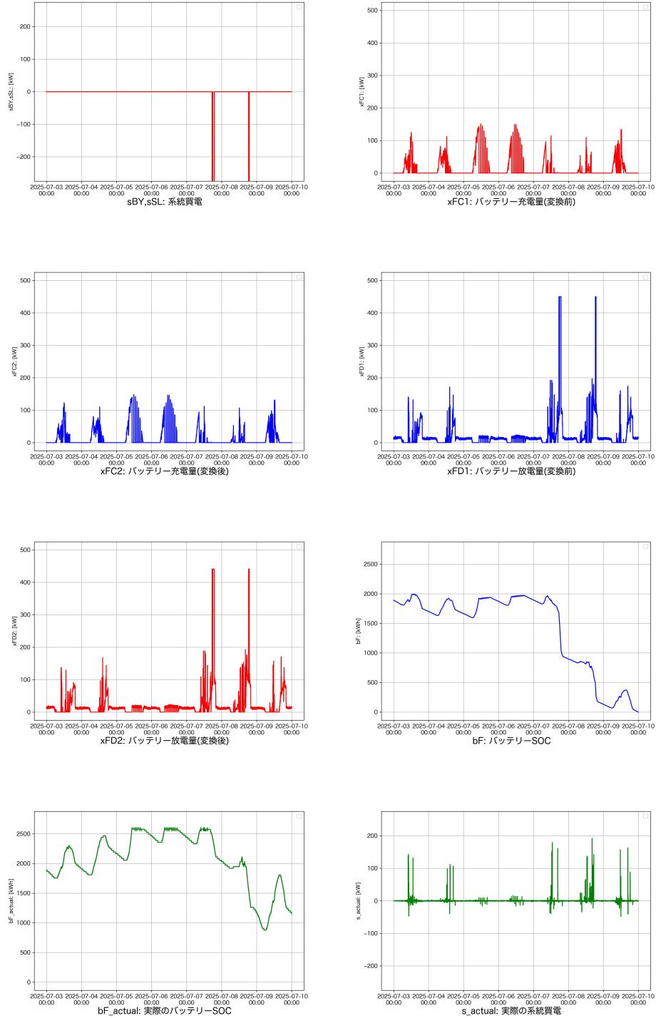
Figure 5.3: Optimization Results (Linear Programming Model) – Page 2
