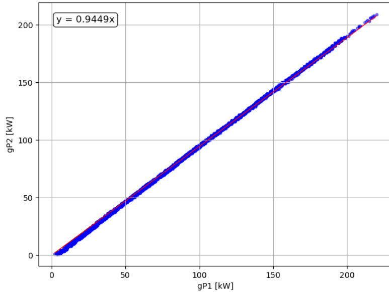
Figure 5.1: Correlation between input and output power in PV inverter
