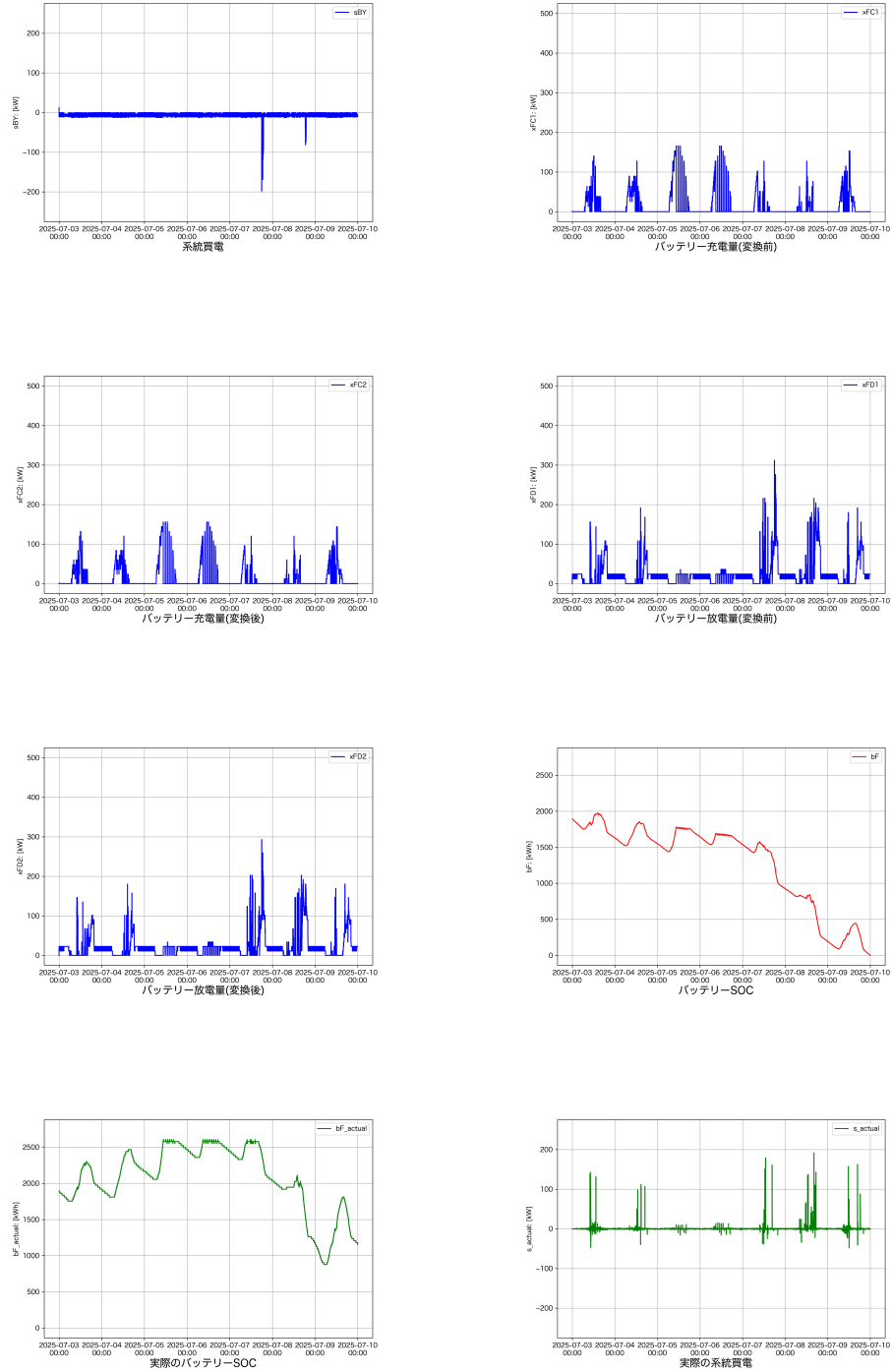
Figure 5.6: Optimization Results (Dynamic Programming Model) – Page 2
