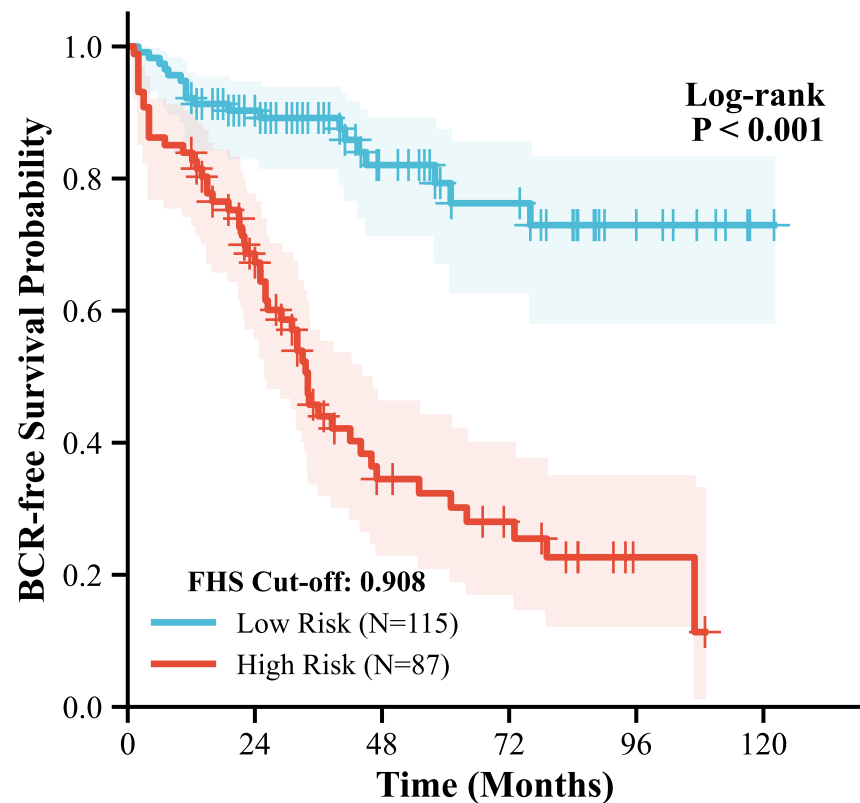
Training
