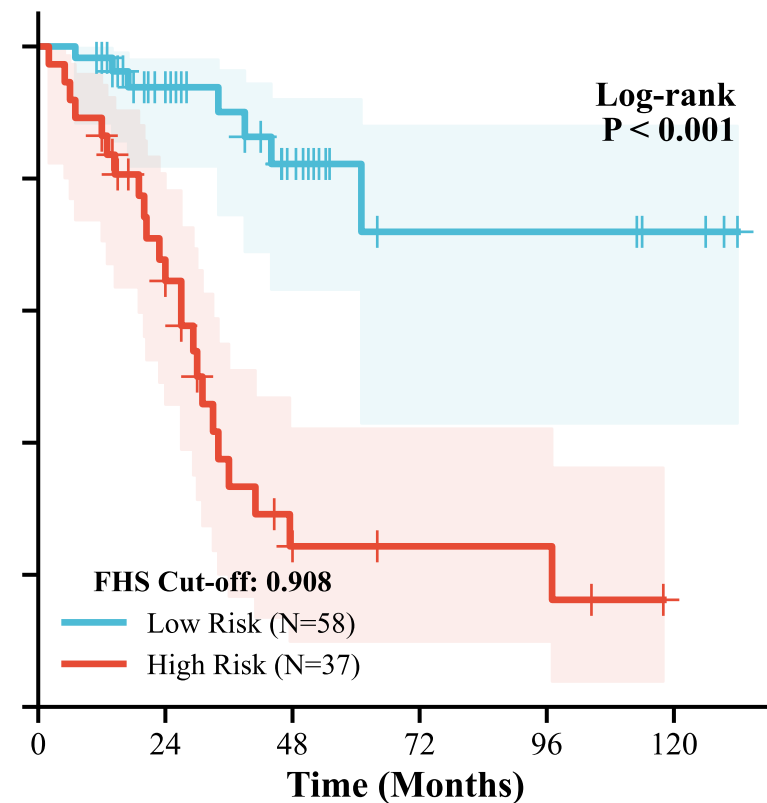
External_Val
