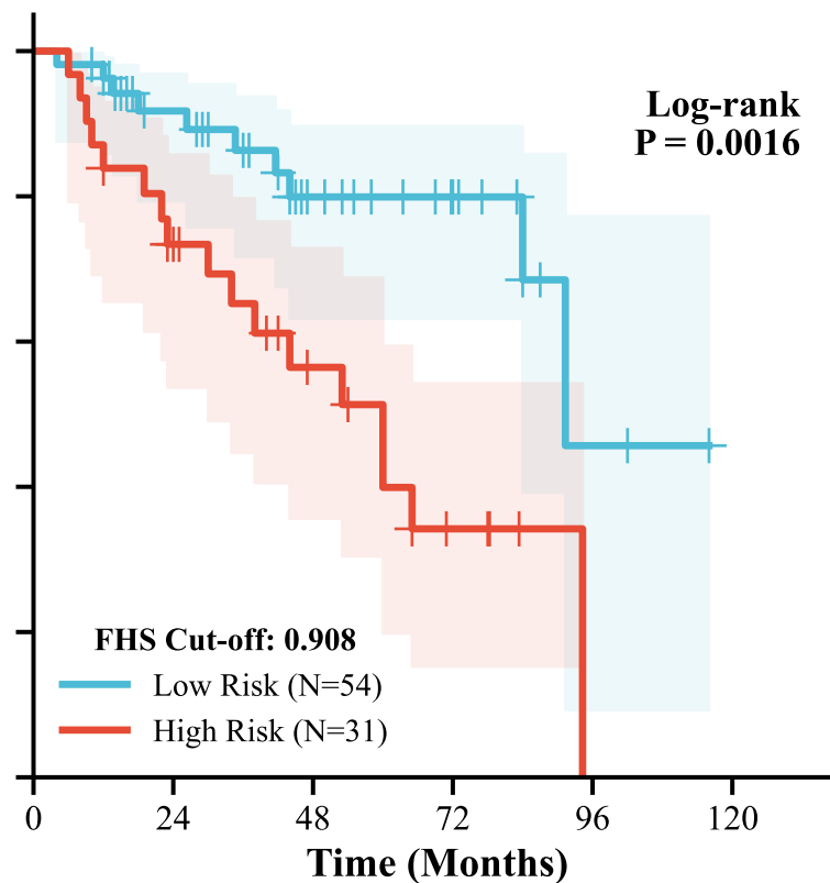
Internal_Val
