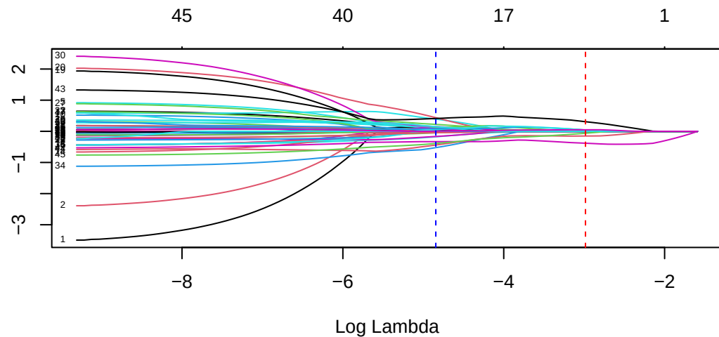
Coefficient Path
