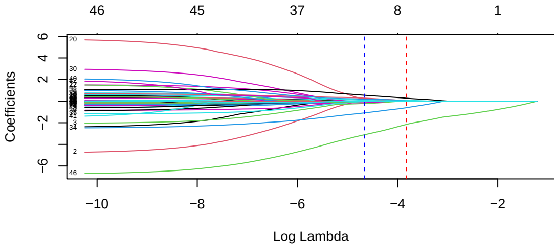
Coefficient Path
