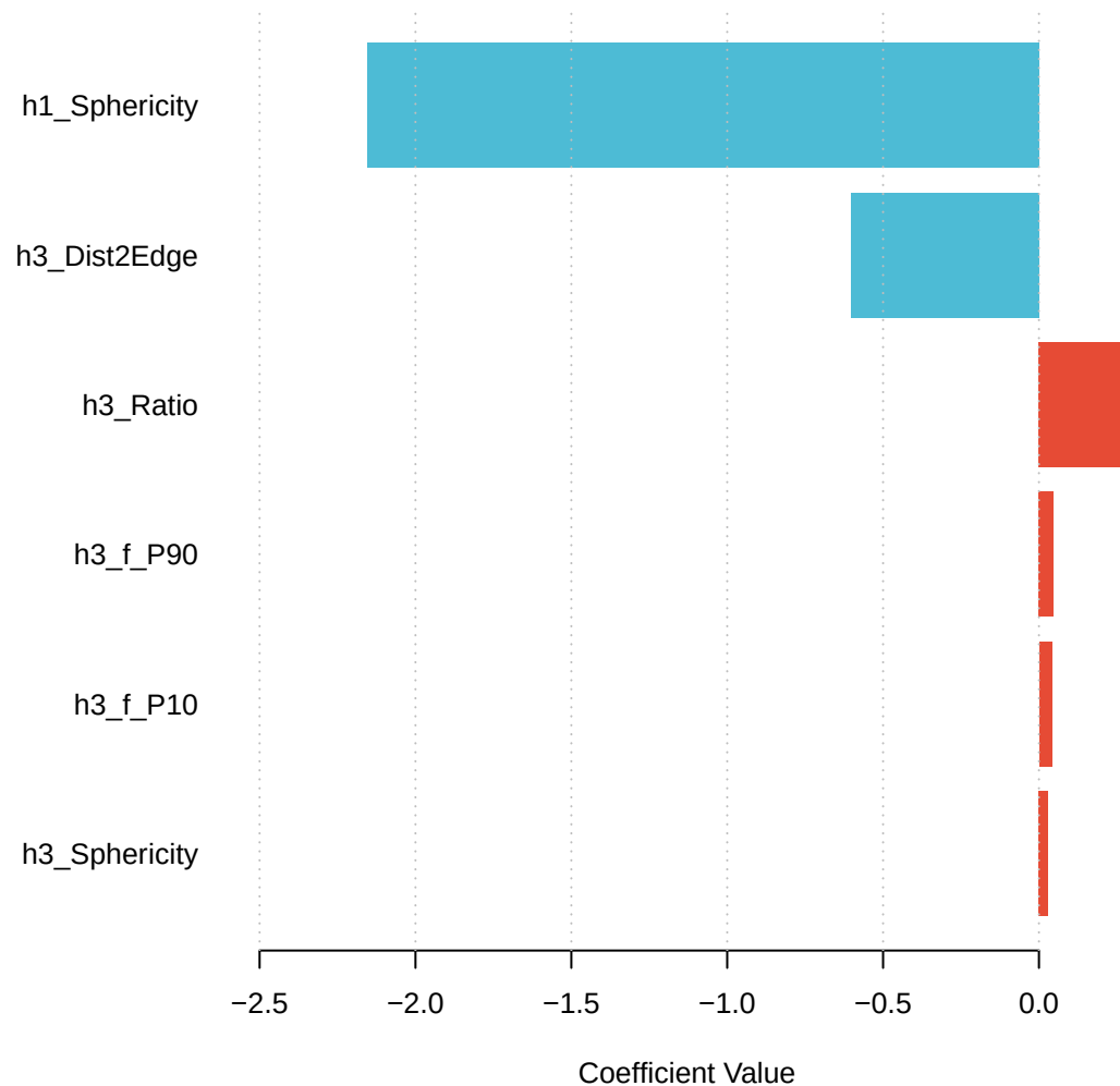
Feature Importance
