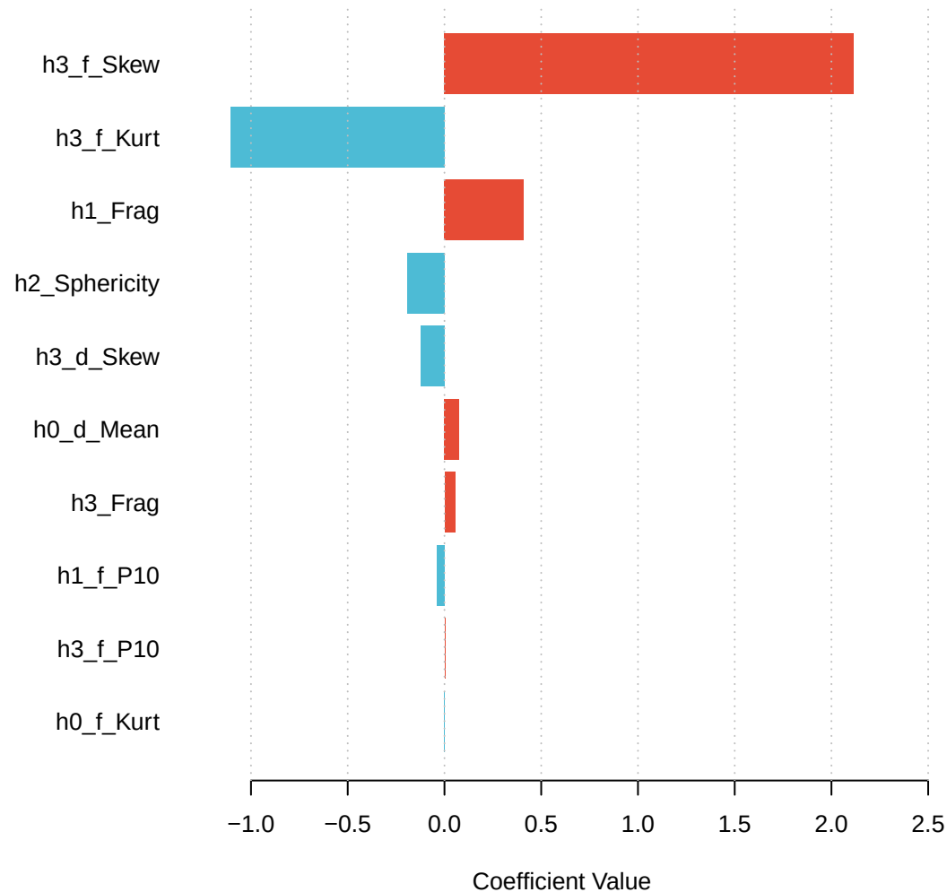
Feature Importance
