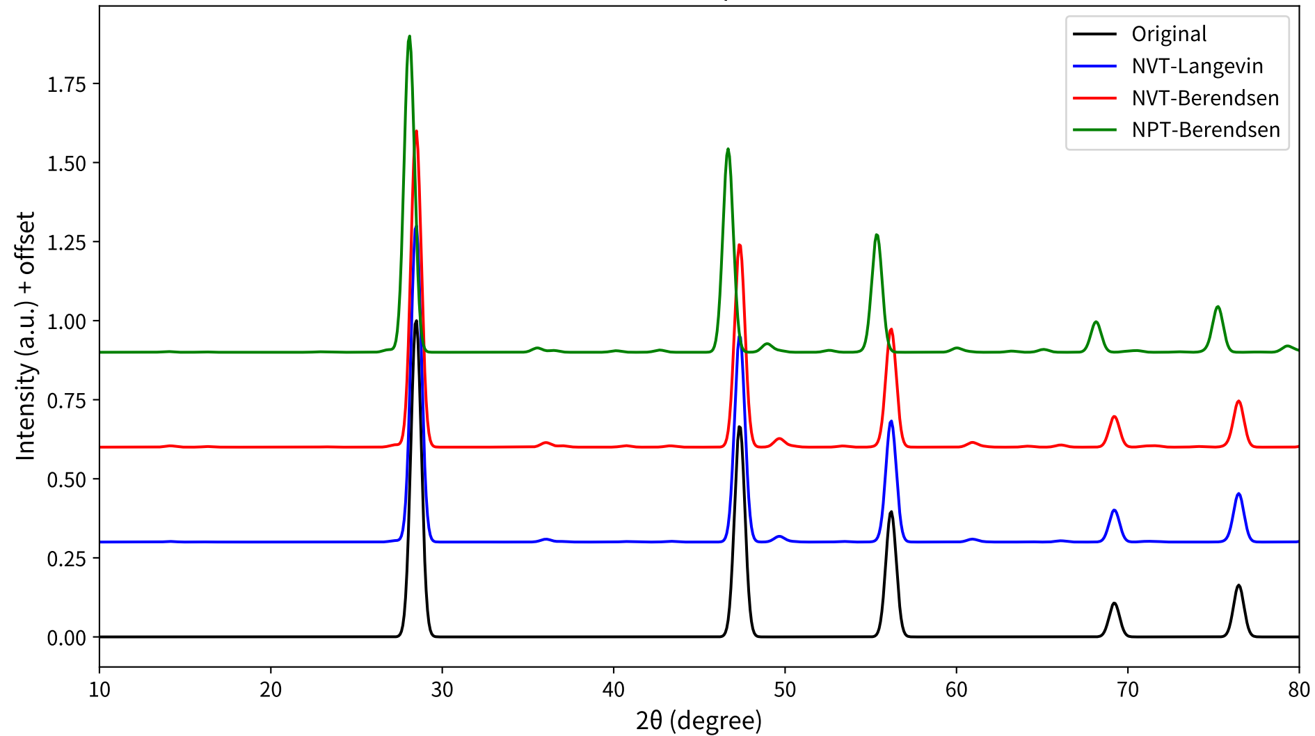
Si XRD: MD Methods Comparison (MACE, 300K)
