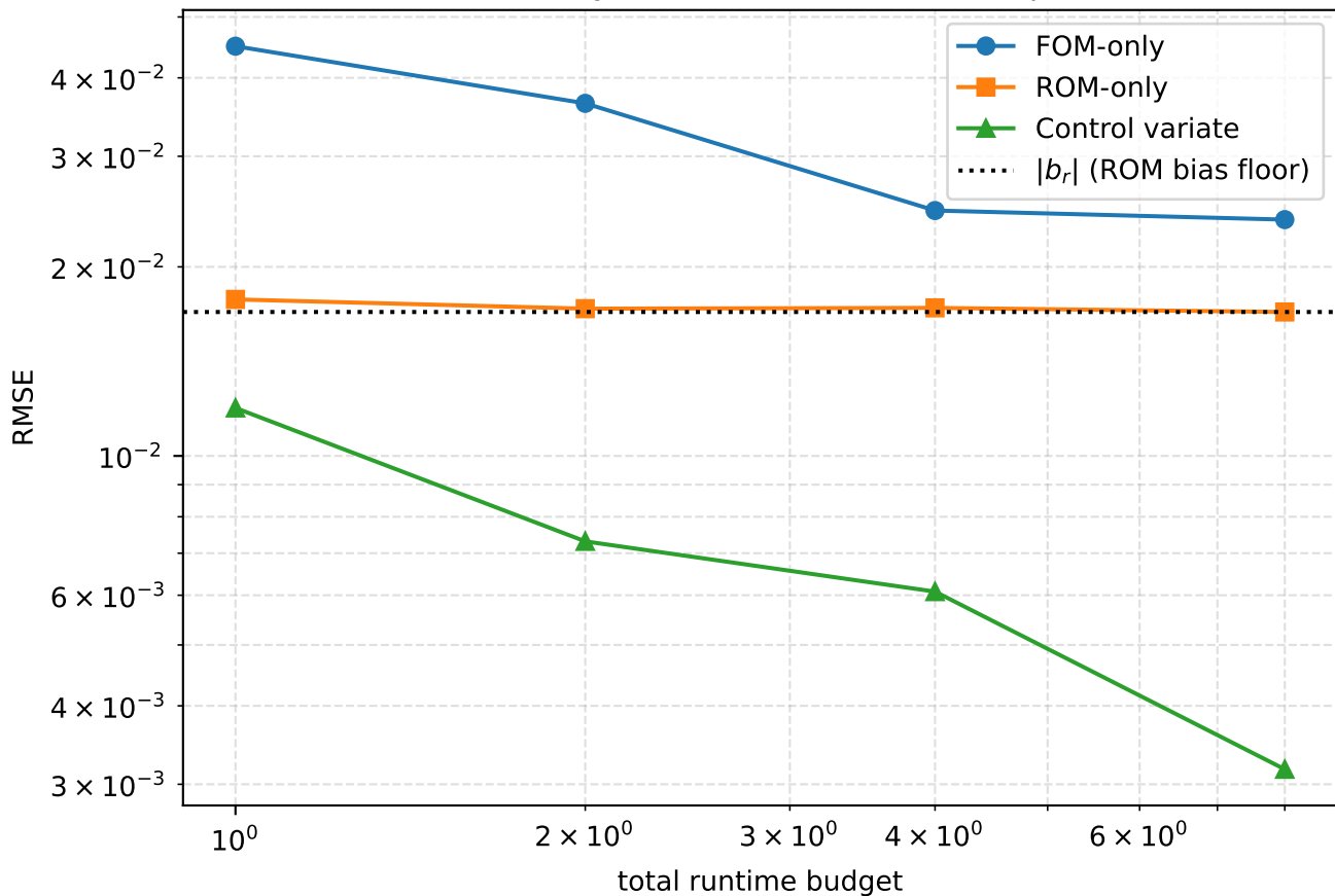
Multi-fidelity RMSE vs runtime (resampled)
