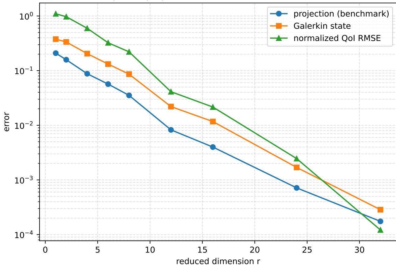
p = 9 : projection, state, and QoI errors vs r
