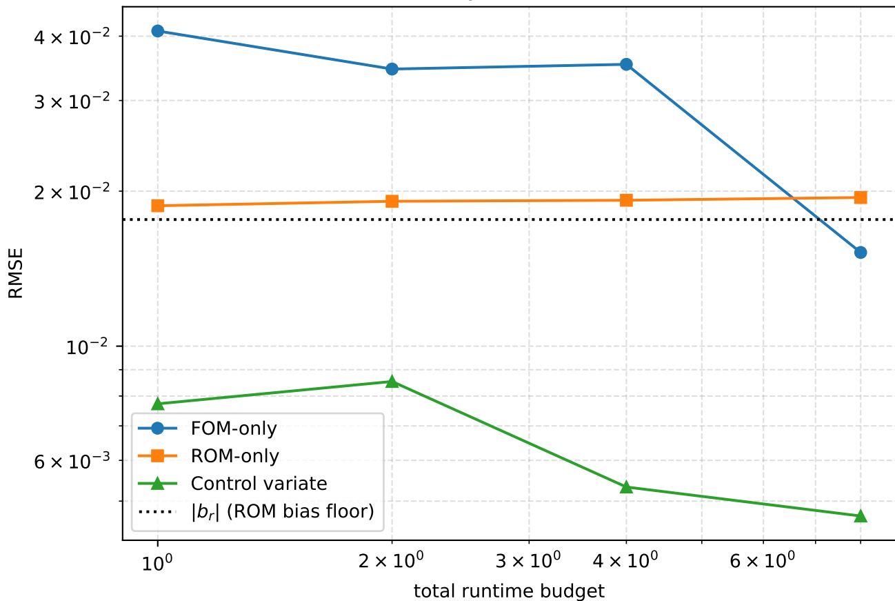
Multi-fidelity RMSE vs runtime
