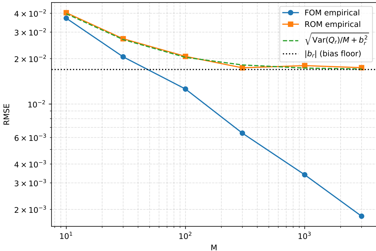
FOM vs ROM Monte Carlo: RMSE vs M
