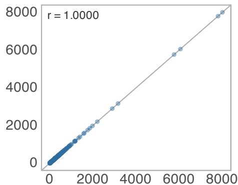
n_words
