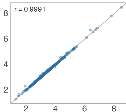
entropy
