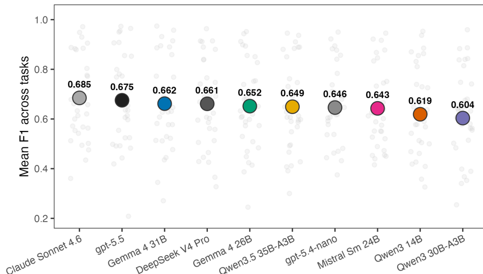
Figure 1: Mean F1 across thirty-three tasks per model. Large filled circles show 33-task means. Small gray dots show observed per-task main F1 values.
