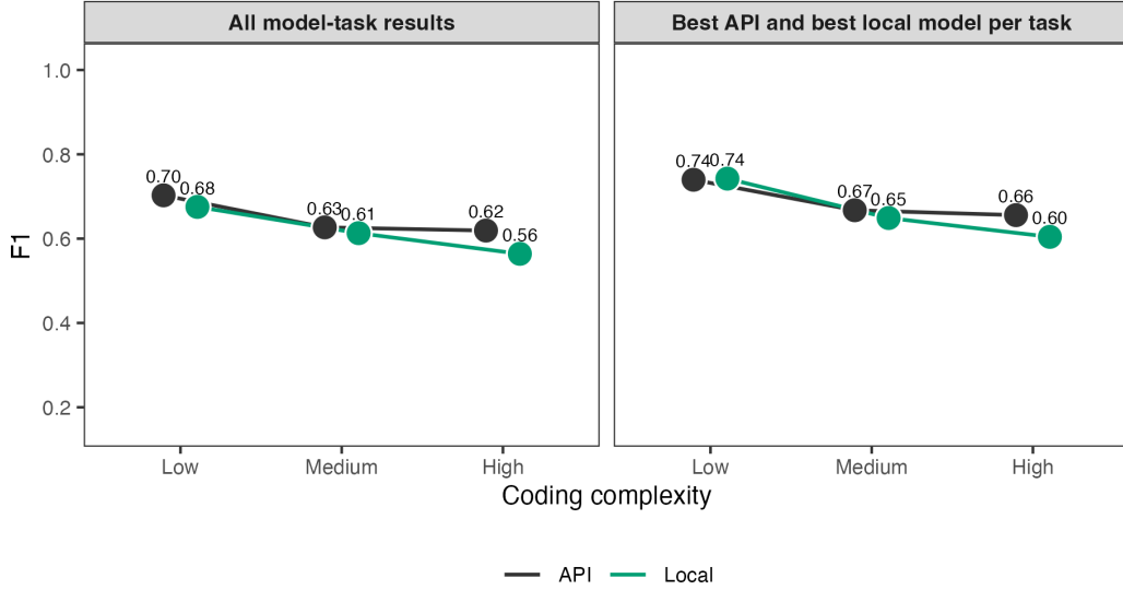
Figure 4: Coding complexity and model performance across the 33-task benchmark. The left panel shows mean F1 across all model-task results, separately for local and API models. The right panel shows the best local model and best API model per task within each complexity group. Points show group means; lines connect complexity groups within model class.
