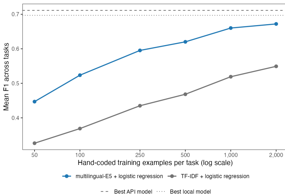
Figure 7: Mean F1 against the number of hand-coded training examples per task, for two supervised classifiers, with the zero-shot LLM results as horizontal reference lines. Points are means over 30 tasks and five random training draws. The reference lines select the best model within each class per task, matching the oracle comparison used earlier.
