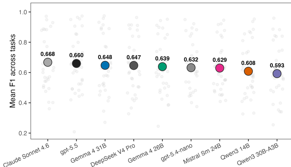
Figure 1: Mean F1 across thirty-four tasks per model. Large filled circles show 34-task means. Small gray dots show observed per-task mean F1 values.
