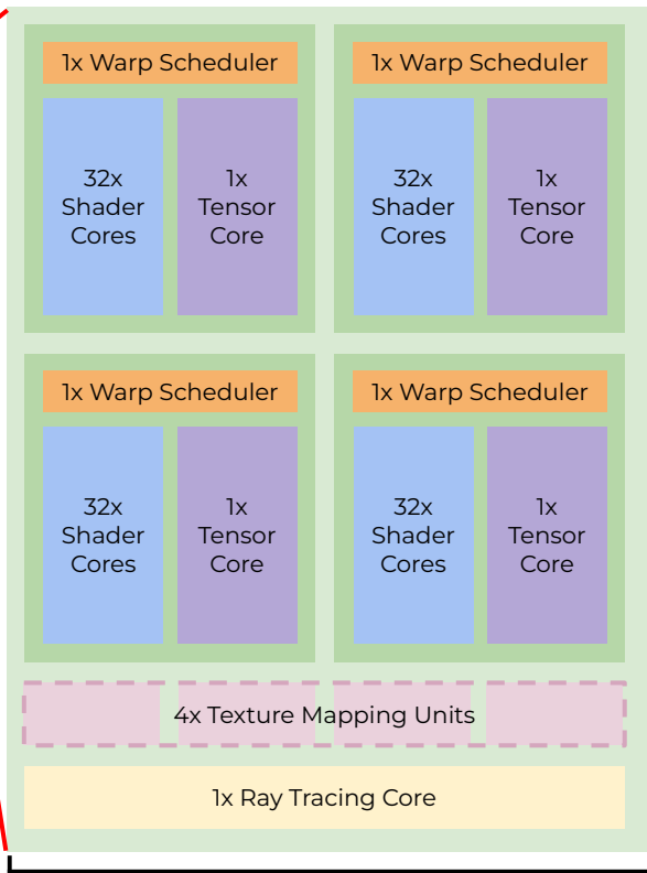
Streaming Multiprocessor
